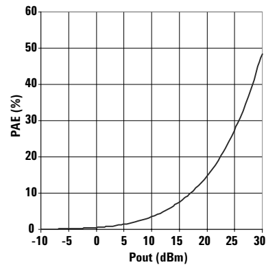
Figure 1. PAE vs Pout
