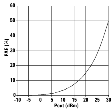
Figure 6. PAE vs Pout
