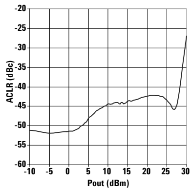
Figure 13. ACLR1 vs Pout
