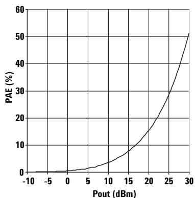
Figure 11. PAE vs Pout
